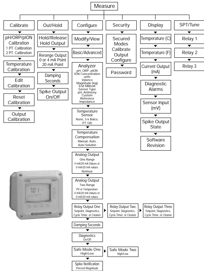
Flow Tree for the TB84pH/ORP/plon Advantage Analyzer
