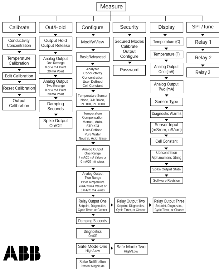
Flow Tree for the TB84TE Two-Electrode Conductivity Analyzer
