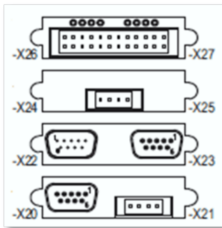
Figure 3: Position of analog and digital outputs
